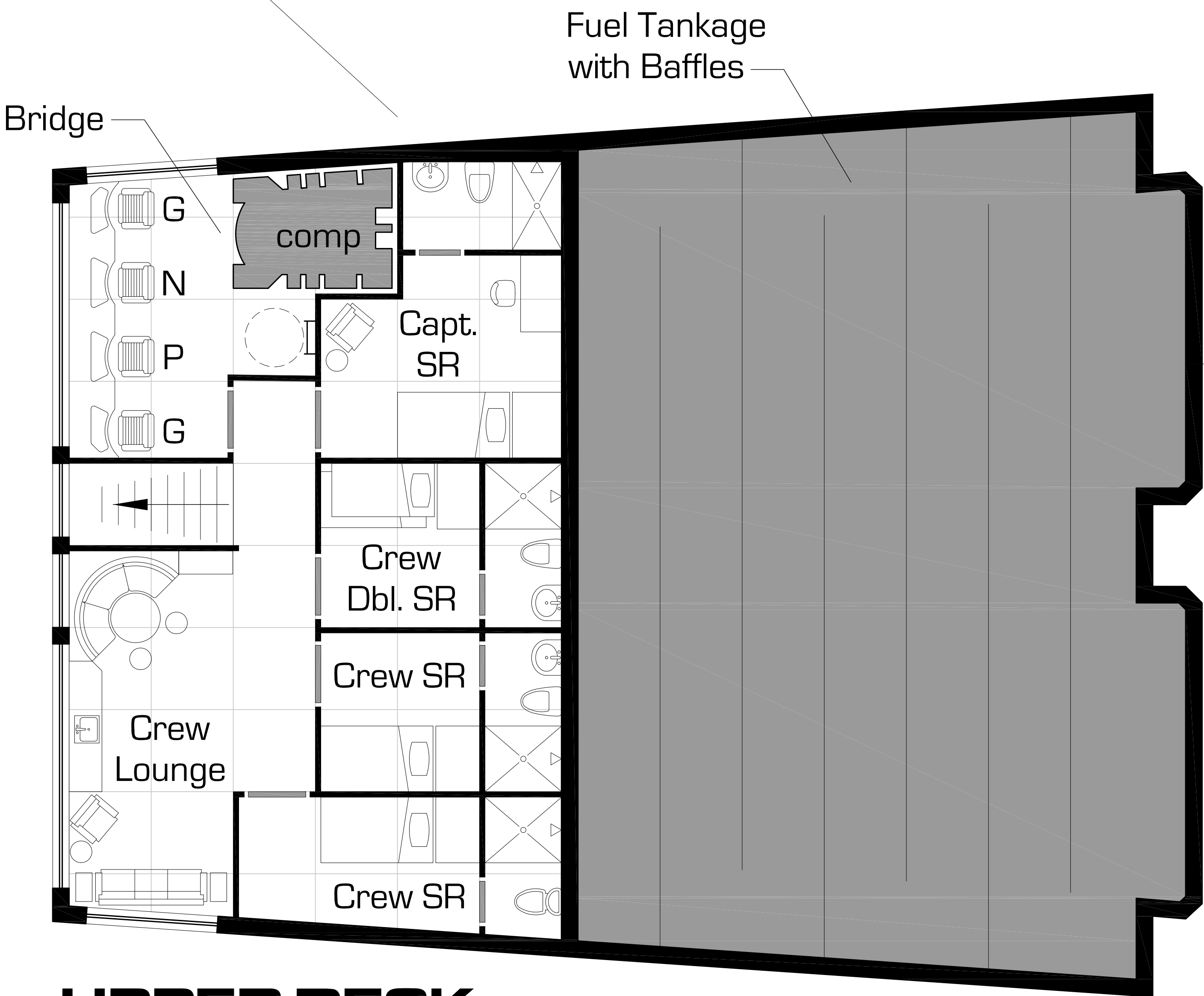
UPPER DECK
