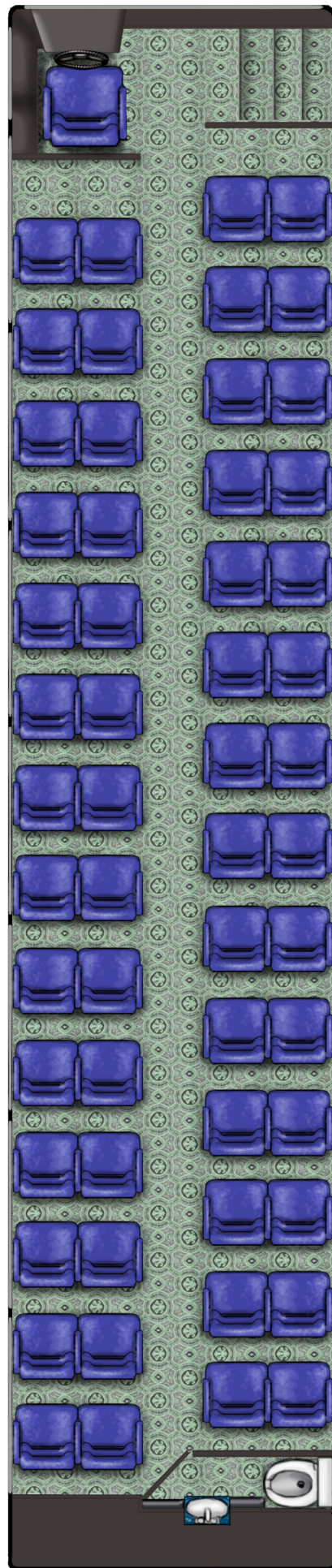
Bus Interior Floorplan
