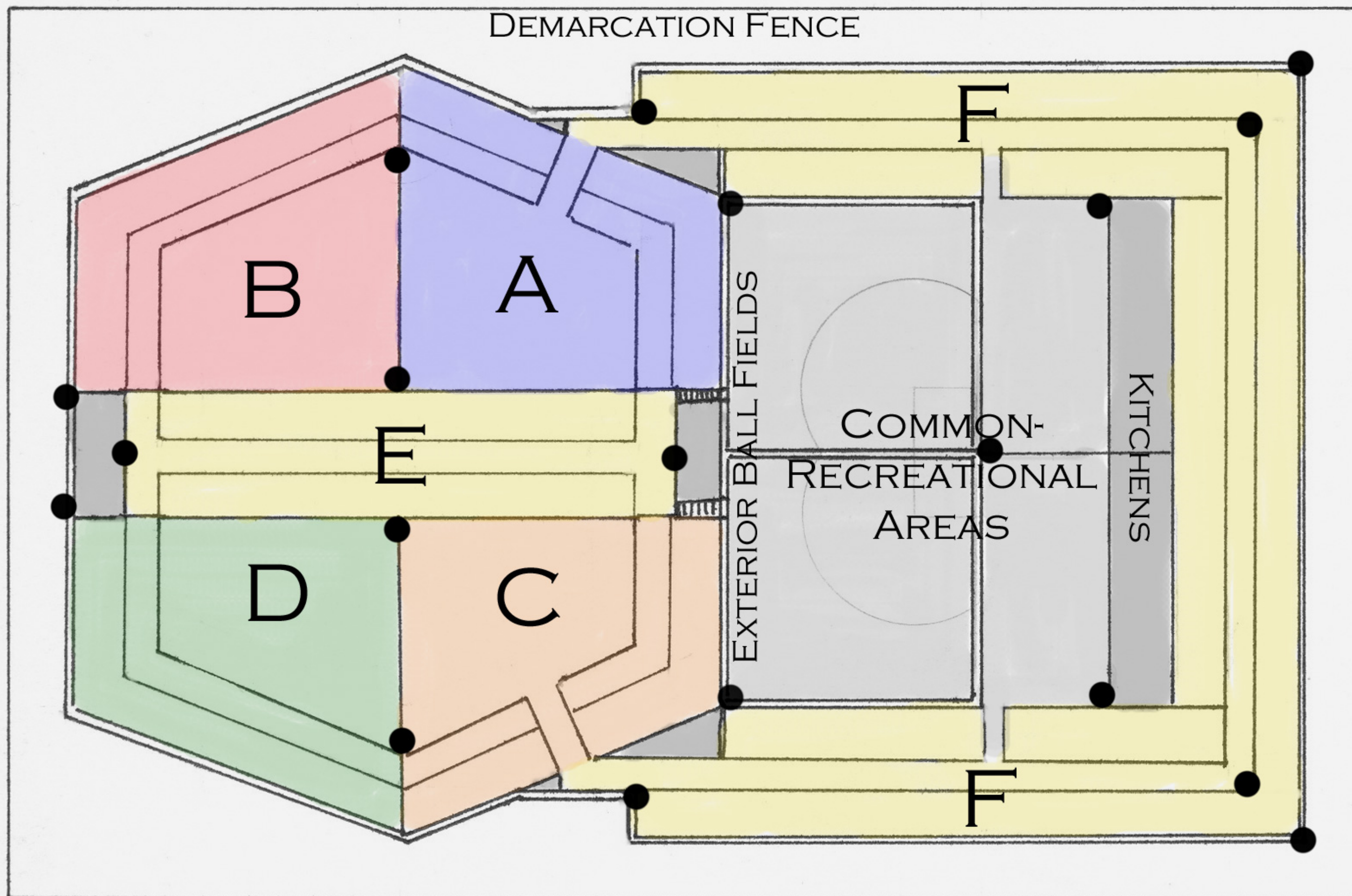
MAIN LEVEL-CELL BLOCKS A-F
