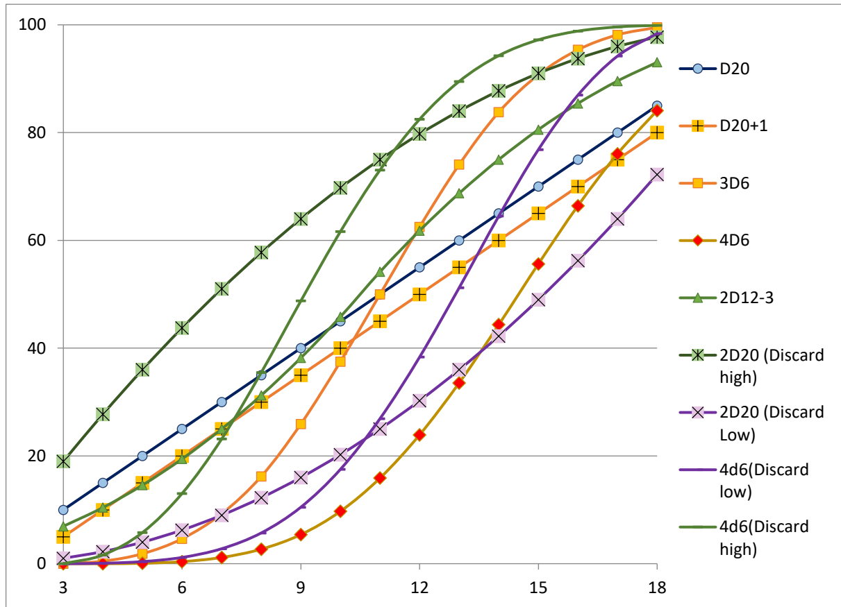
Graph 1 – All the probability 'curves' given together
