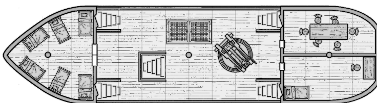
MAIN DECK
